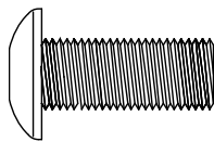
#32. 5/16" × 3/4" Button Head Socket Bolt (4 pcs)
